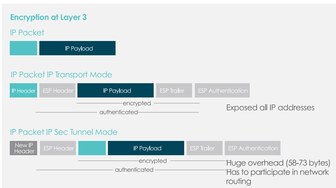
Figure 2 – IPSec encryption overhead
