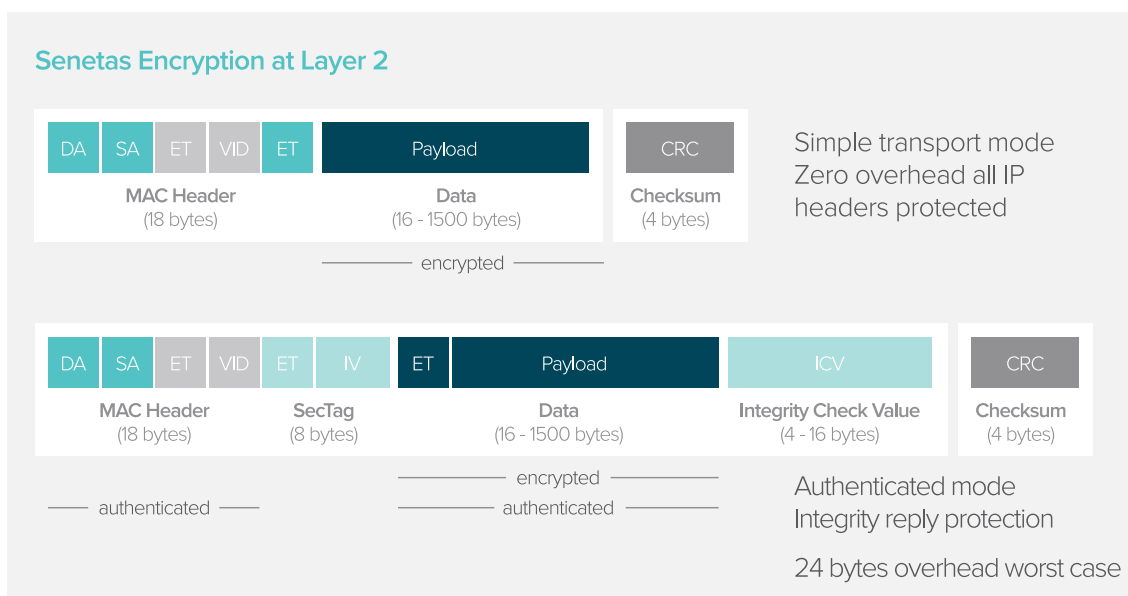
Figure 3 – Ethernet encryption overhead
